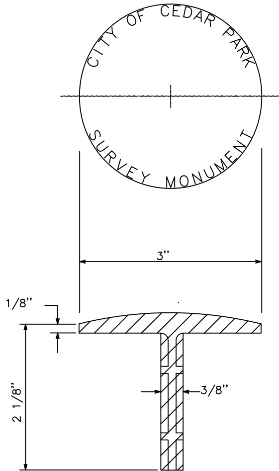
CROSS SECTION MONUMENT, TYPE C MATERIAL: ONE PIECE CAST BRASS
