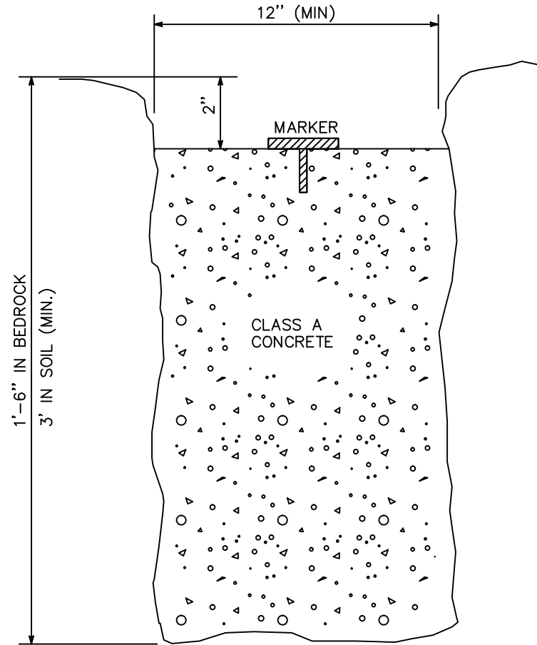
SURVEY IDENTIFICATION MARKER NON TRAFFIC CONSTRUCTION DETAIL
